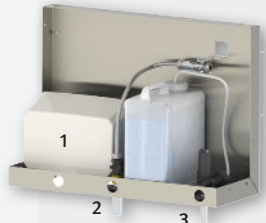
Modular system including high speed hand dryer (1), touch free faucet (2) and liquid soap dispenser (3)
